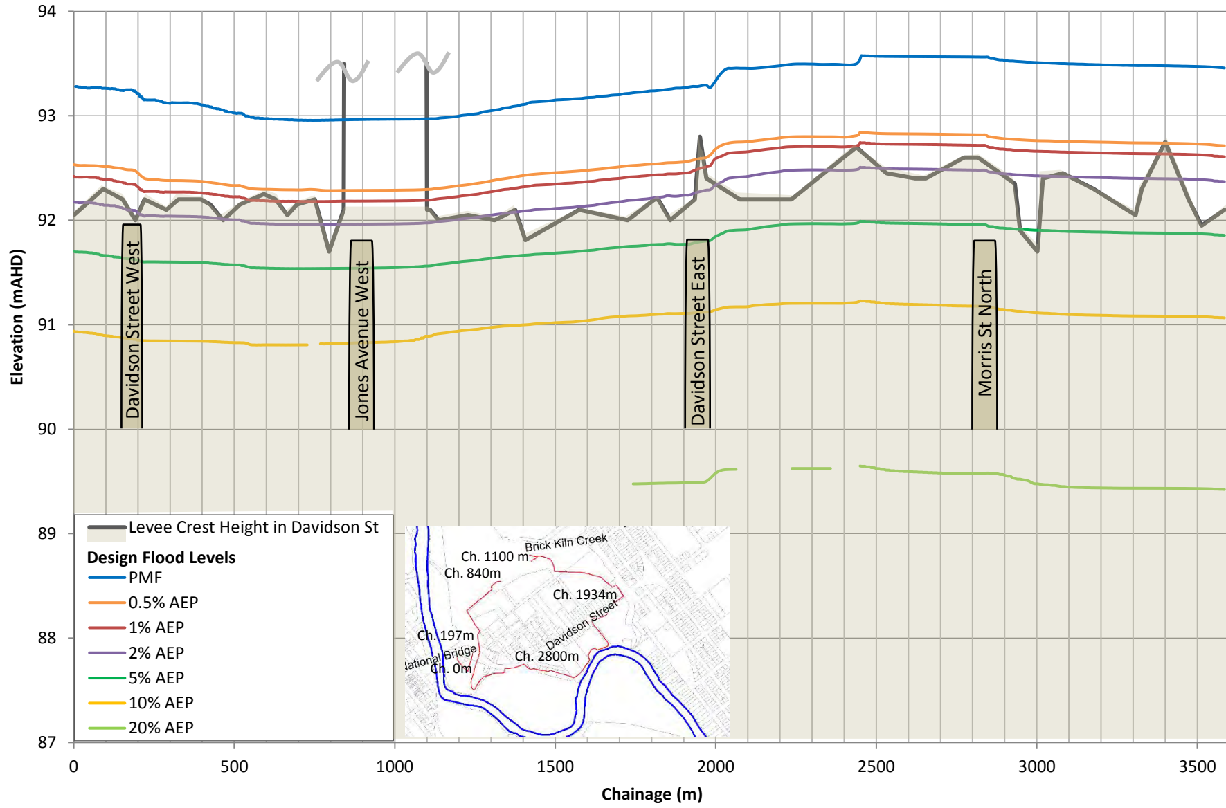
DAVIDSON STREET LEVEE DESIGN FLOOD EVENT PROFILE FIGURE 13
