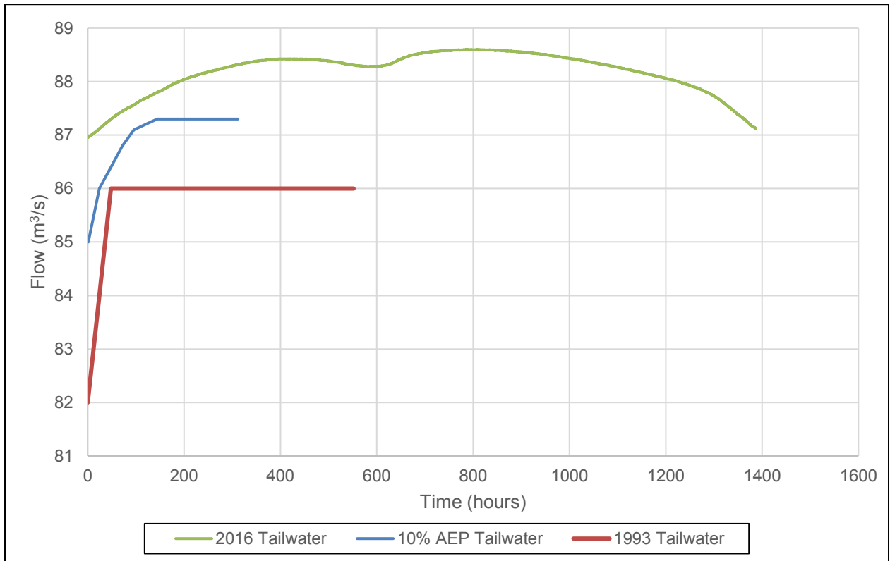
Chart 8: Model Tailwater Comparison
