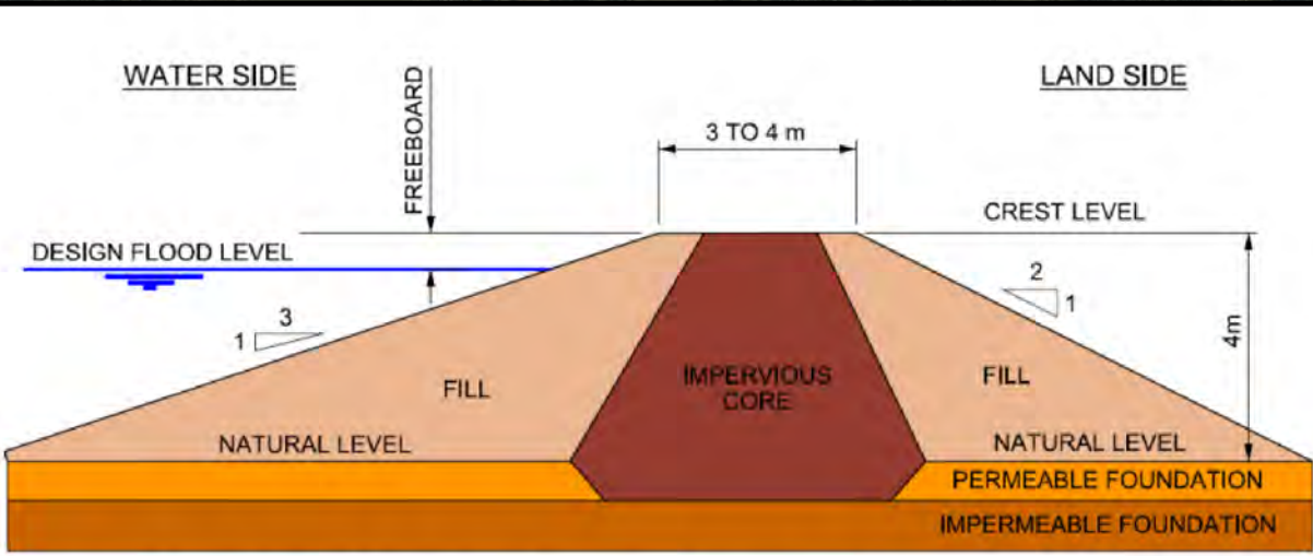
Figure 4.1 Typical NSW earth embankment levee cross section
