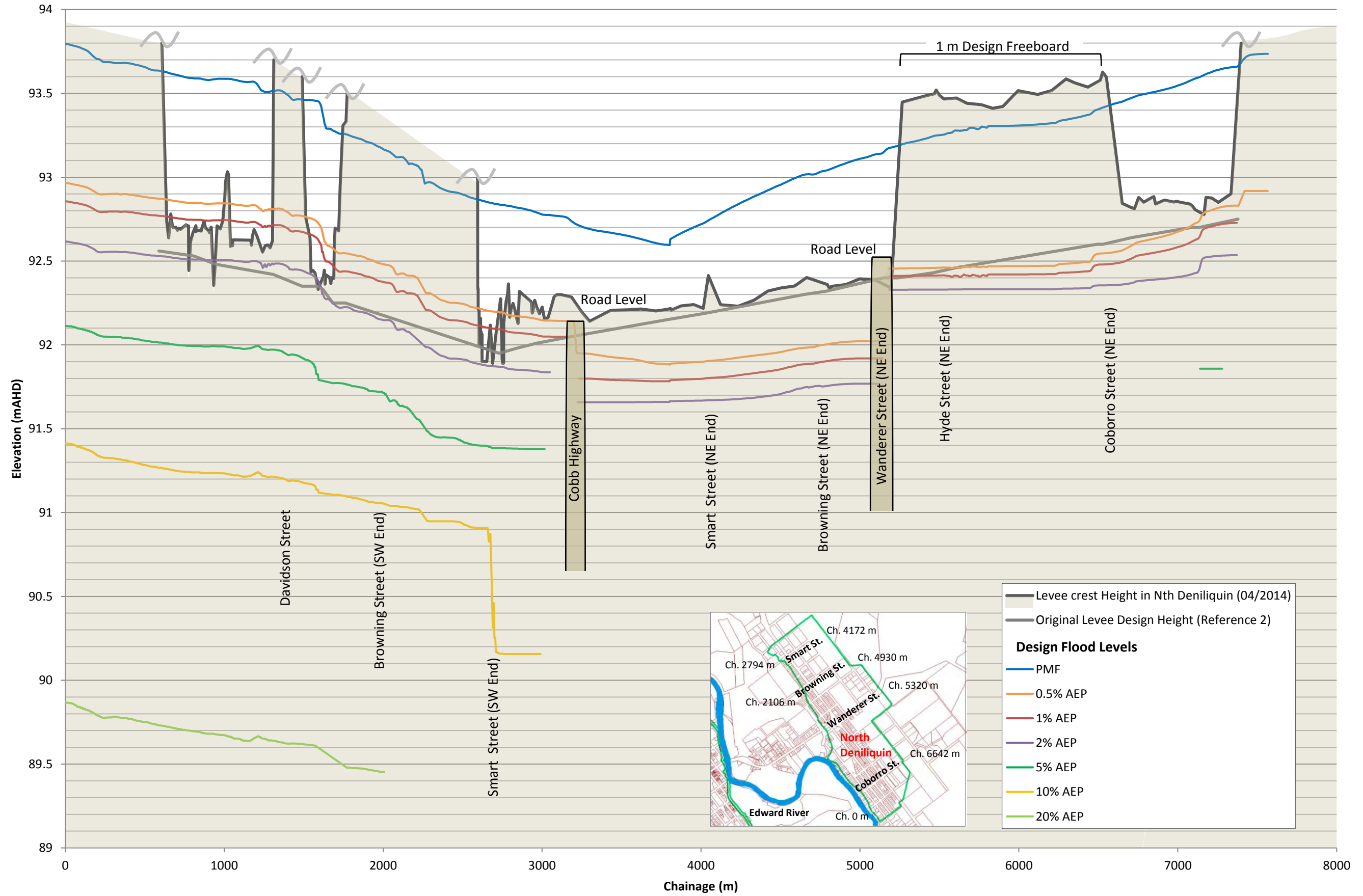
FIGURE 12 NORTH DENILIQUN LEVEE DESIGN FLOOD EVENT PROFILE
