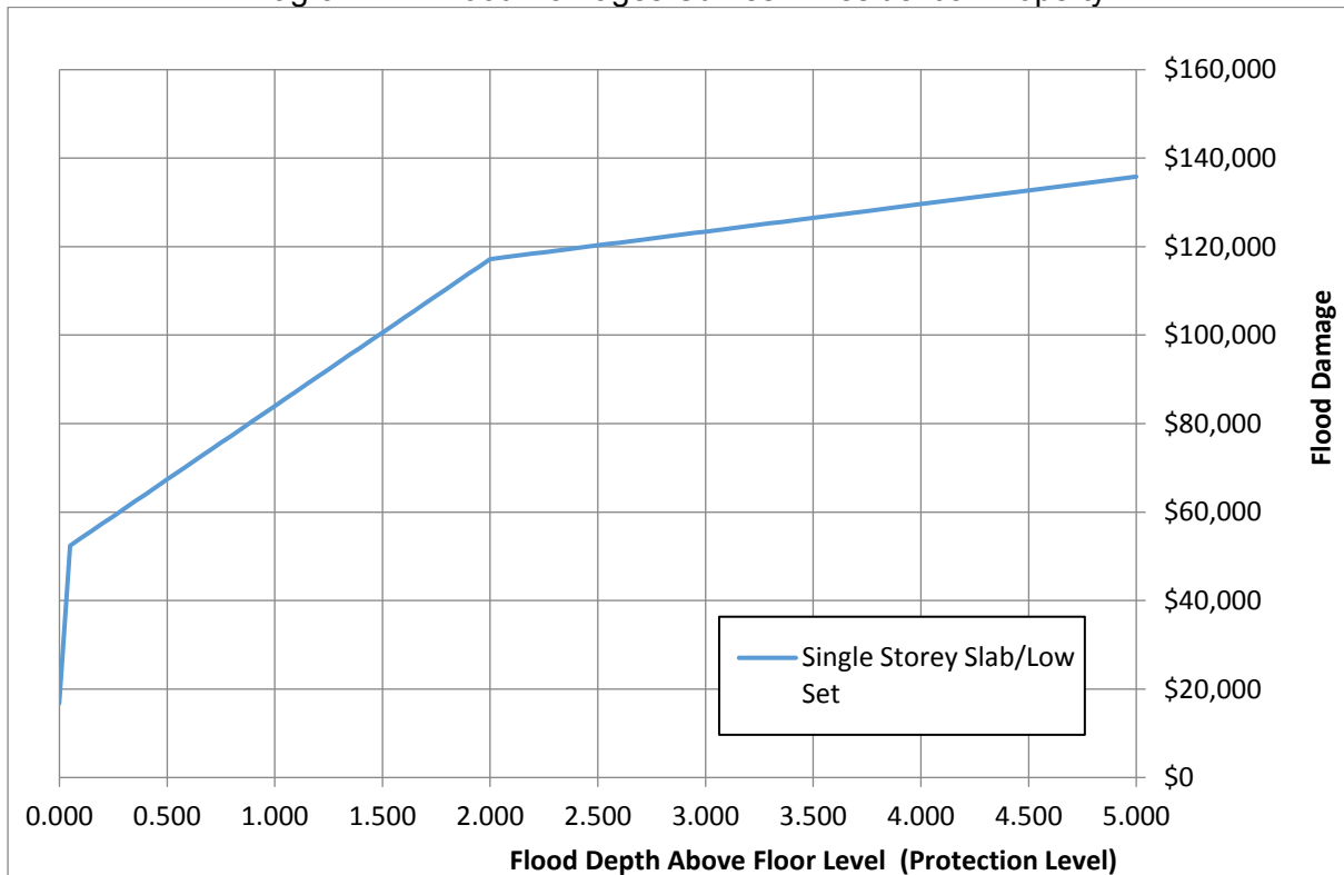
Diagram D2: Flood Damages Curves – Residential Property
